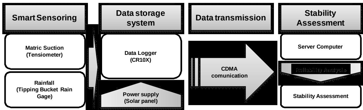
Fig.2 Schematic diagram of probabilistic smart monitoring system
