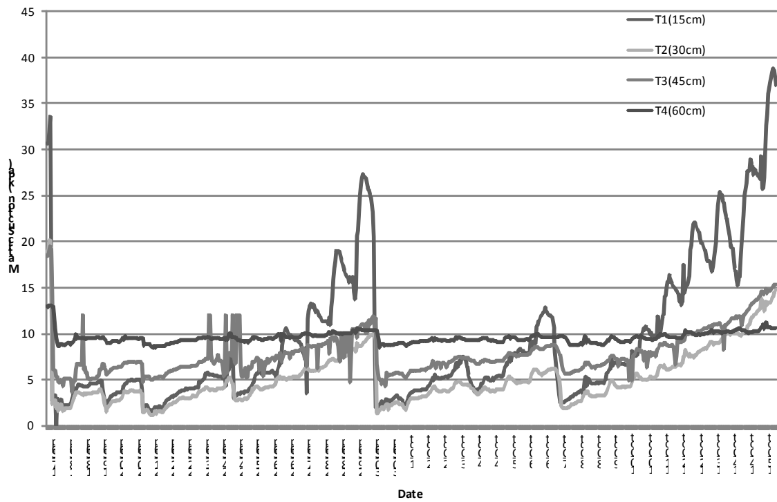
Fig.4 Measured matric suction during monitoring
