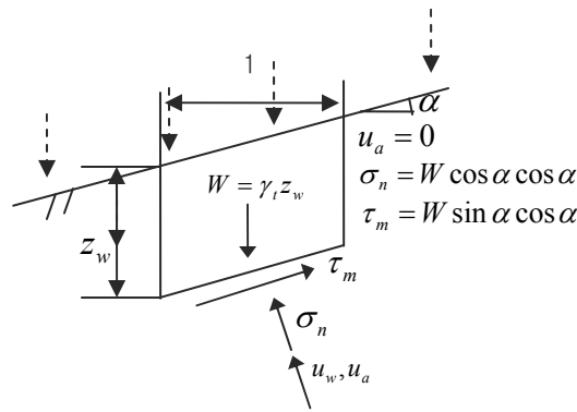
Fig.1 Infinite slope stability
