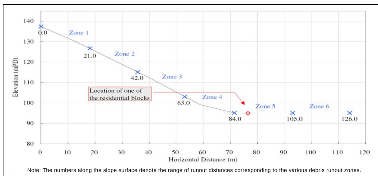
Fig.4 Debris Runout Zones of Segment 5e
