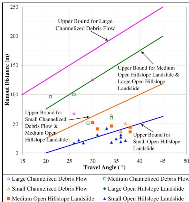
Fig.3 Landslide Debris Runout Model
