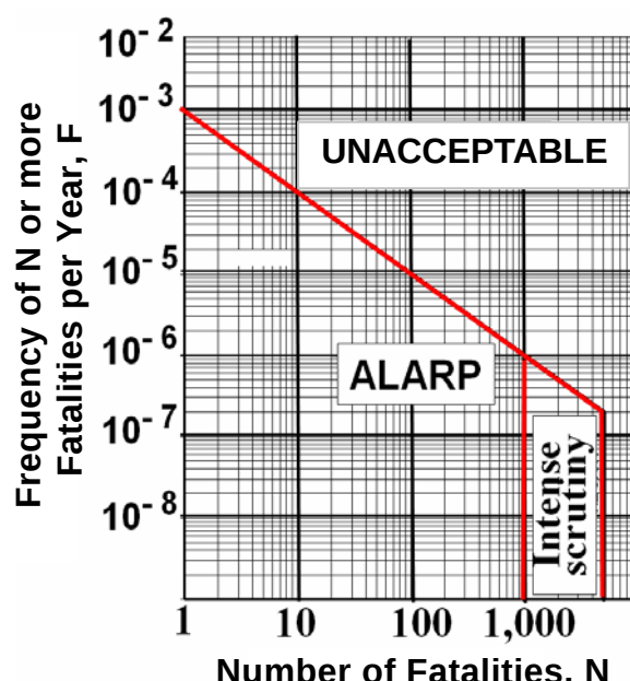
Fig.2 Societal Risk Criteria Adopted by the Government of the Hong Kong SAR for Natural Terrain Landslide Hazards
