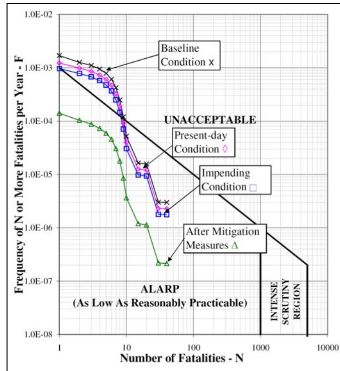
Fig.5 Societal Risk of Different Conditions in F-N Curves
