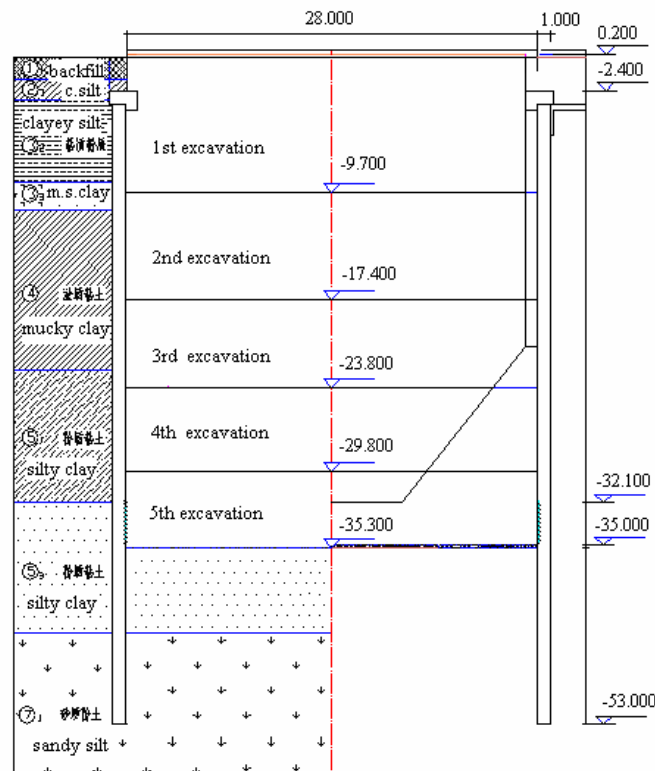
Fig.3 Scale pit elevation section
