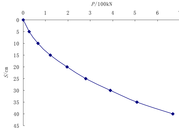
Fig.3 P-S curve
