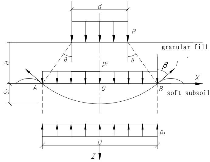
Fig.1 Model for geogrid-reinforced unpaved road
