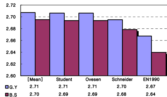
(b) Specific gravity
