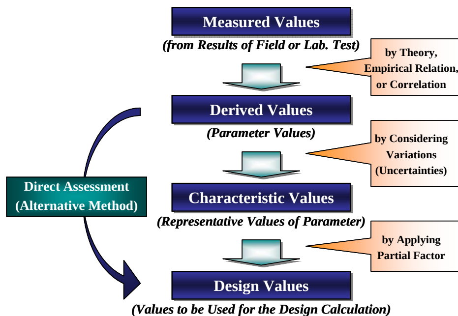
Fig.1 Procedure to determine design value (Orr et al., 1999)
