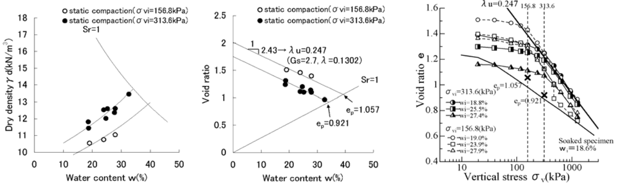
(a) Compaction curves (dry density) (b) Compaction curves (void ratios) (c) Compression curves Fig.4 Relationship between compaction curves and compression curves (Honda et al. 2007)
