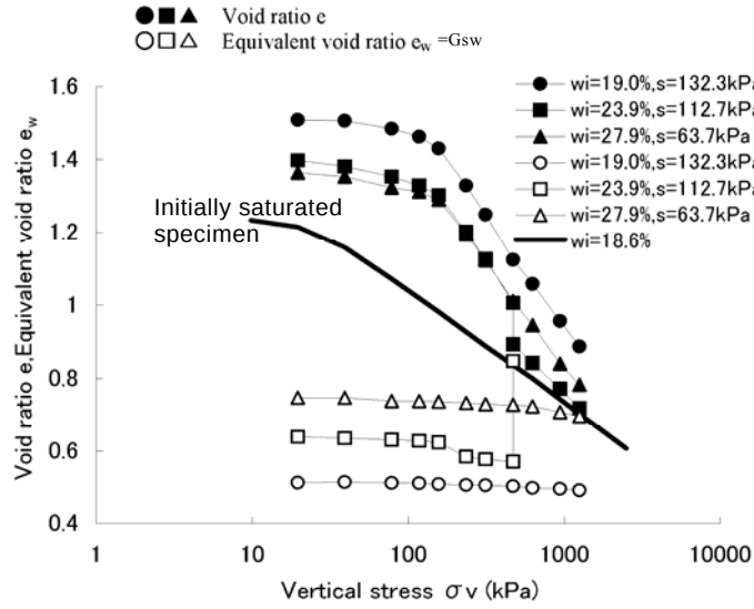
Fig.1 Compression curves of silt (Honda et al.2006)
