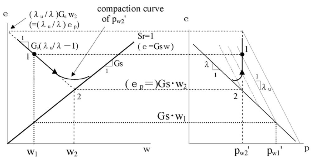
Fig.3 Relationship between compaction curves and compression curves (Honda et al.(2007))
