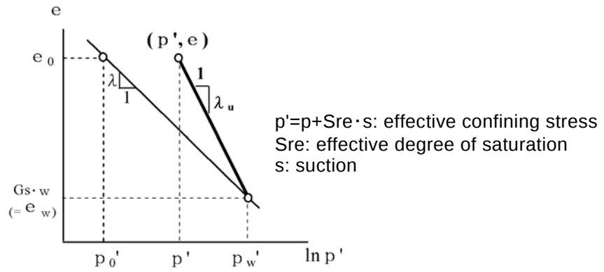
Fig.2 Conceptual compression curves
