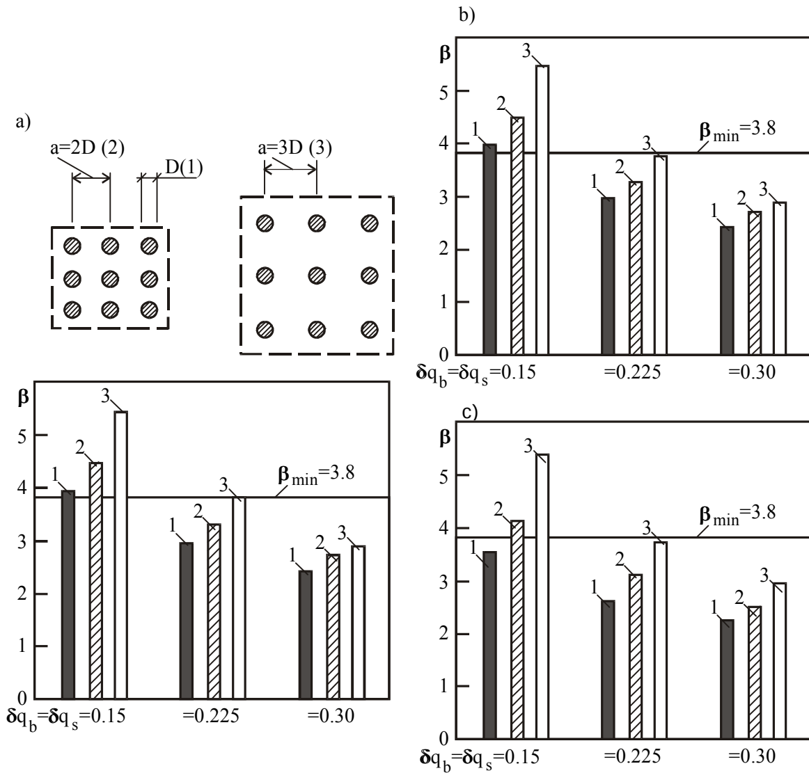
Fig.3 The external reliability index \beta by (20) versus the coefficient of variation \delta q of cohesionless soil resistances for single piles (1) and pile blocks with a/D=2 (2) and a/D=3 (3) in the absence (a) and presence of sustained (b) and extraordinary (c) variable actions
