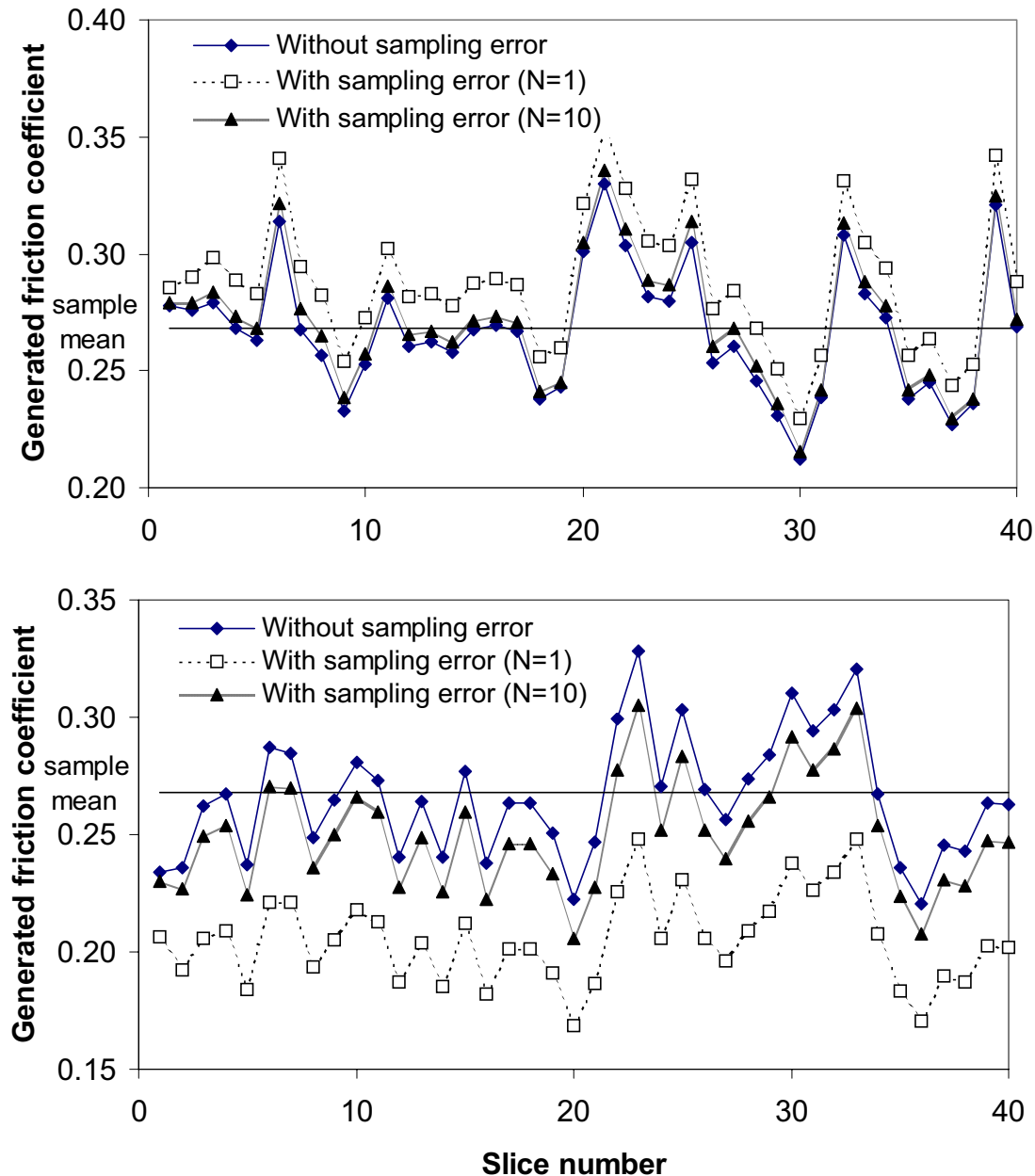
Fig. 5 Samples of Generated Friction Coefficients over the 40 Slices of the Slip Surface: (a) with Trend Higher than the Sample Mean; (b) with Trend Lower than Sample Mean; N: Number of Samples
