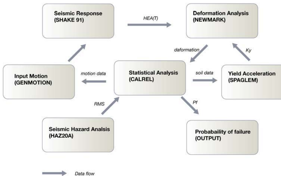
Fig. 3 Numerical Implementation and Data Flow of Probabilistic Seismic Slope Deformation Analysis
