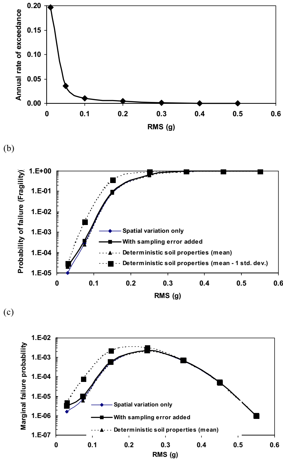
Fig. 7 (a) Annual Hazard Curve (Annual Rate of Exceeding Each Hazard Level); (b) Fragility Curve; (c) Marginal Annual Risk Curve (Annual Probability of Failure with Respect to Each Hazard Level)
