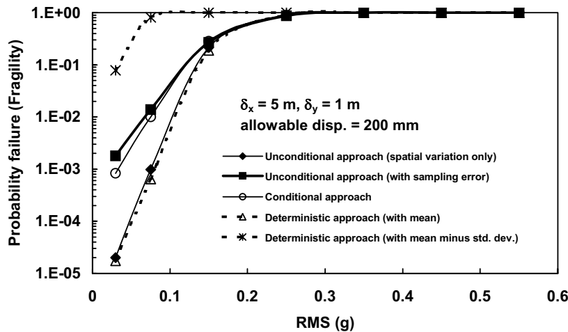
Fig. 9 Probability of Failure Given the Certain Hazard Levels (Fragility Curve)
