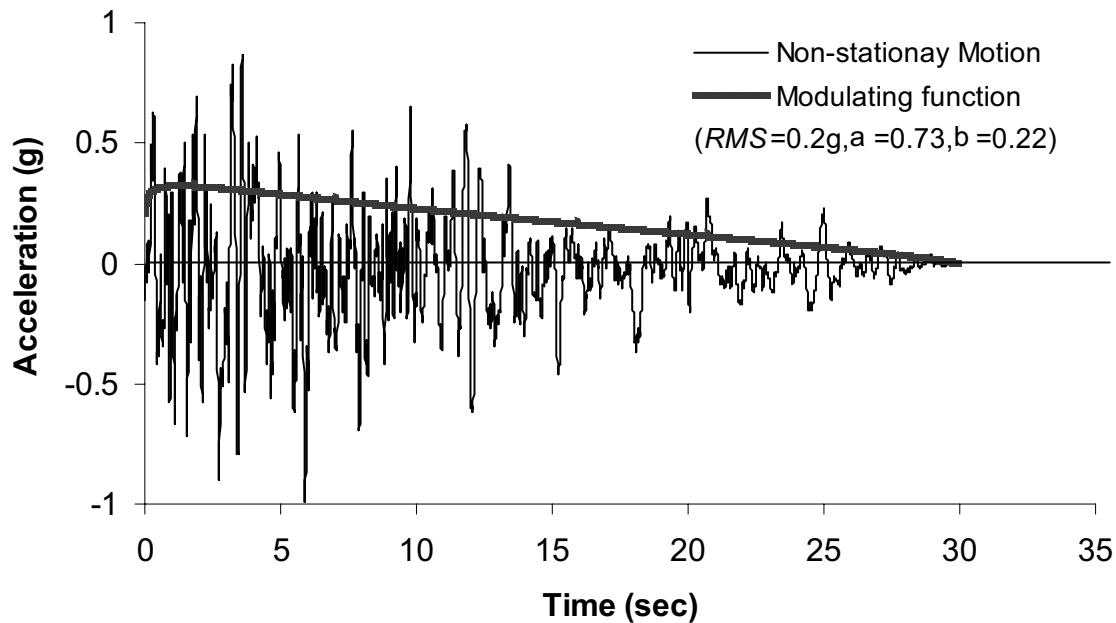
Fig. 2 Sample Time History of Non-Stationary Ground Motion (RMS=0.2 g, a=0.73, b=0.22, td=30 sec)
