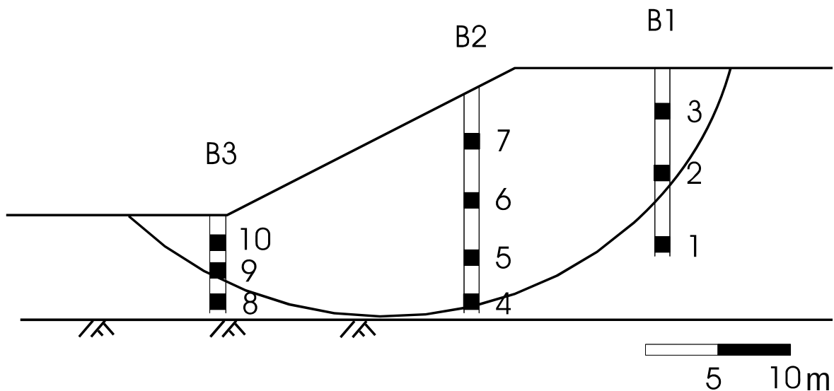
Fig. 8 Geometry and Sample Location of a Slope with a Circular Slip Surface
