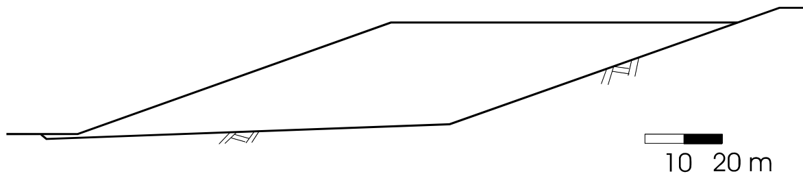
Fig. 4 Geometry of the Landfill Lying on the Gently Sloping Potential Slip Surface
