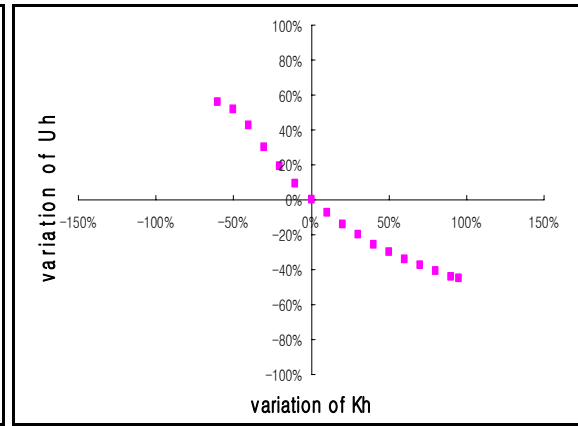
Fig.5 Variation of U_h depending on k_h
