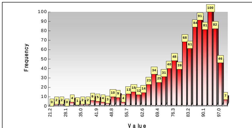
Fig.17 Degree of consolidation distribution for 1.5m installation space
