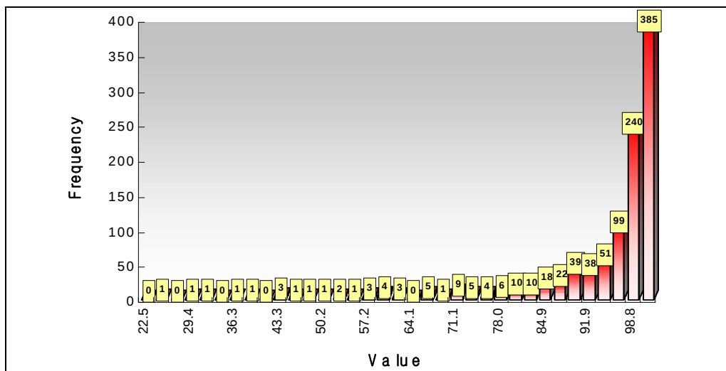
Fig.15 Degree of consolidation distribution for 1.0m installation space
