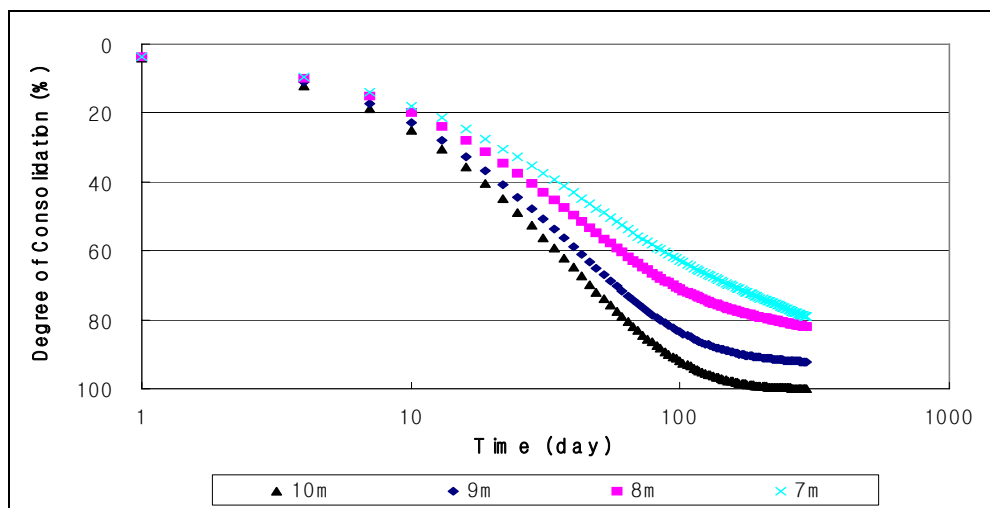
Fig.11 Comparison between complete installation and partial installation with depth
