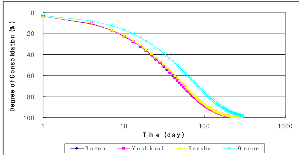
Fig.10 Degree of consolidation with analysis method
