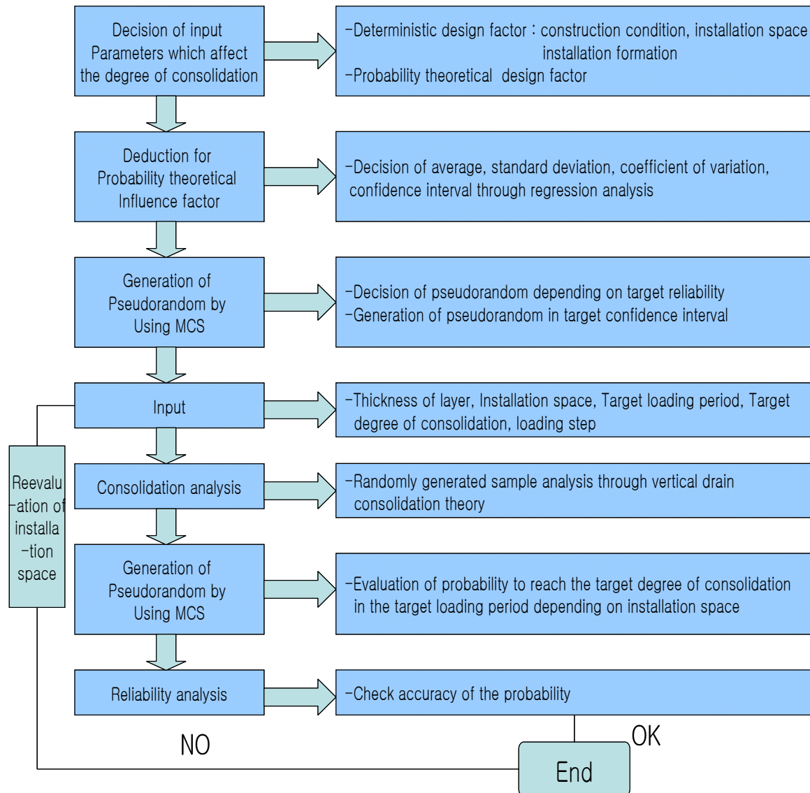
Fig.3 Flow chart of reliability analysis
