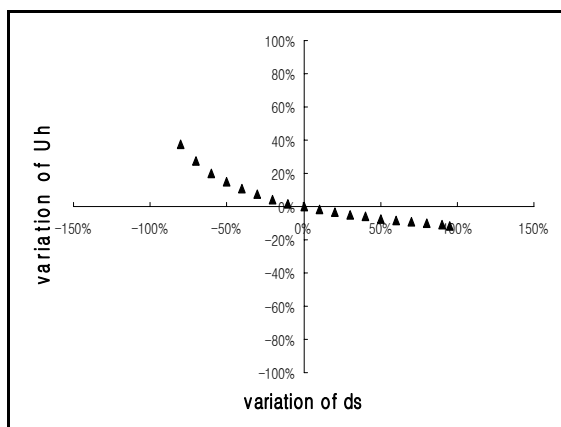
Fig.6 Variation of U_h depending on d_s
