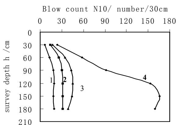
1, Dr=0.49 ; 2, Dr=0.62 ; 3, Dr=0.76 ; 4, Dr=0.93 ; Fig.5 Results of No.4 sand
