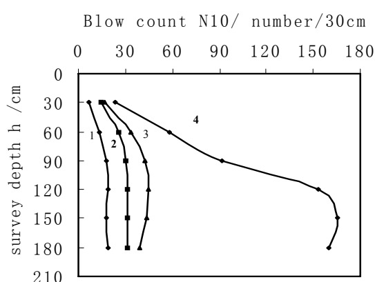
1, Dr=0.49 ; 2, Dr=0.59 ; 3, Dr=0.74 ; 4, Dr=0.90 ; Fig.4 Results of No.3 sand
