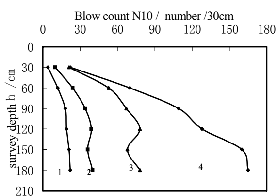
1, Dr=0.54 ; 2, Dr=0.70 ; 3, Dr=0.81 ; 4, Dr=0.89 Fig.2 Results of No.1 sand
