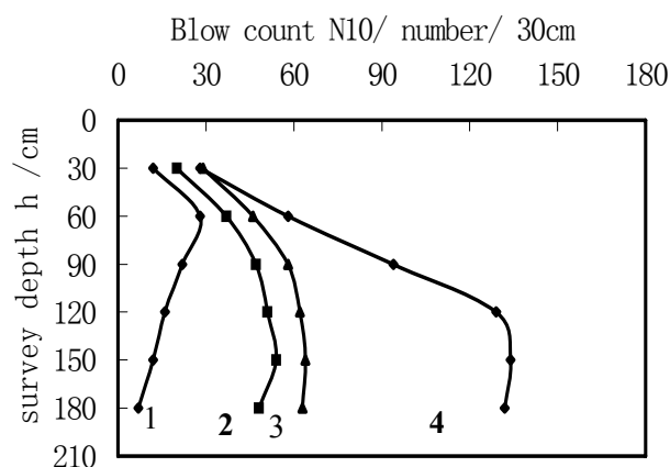
1, Dr=0.49 ; 2, Dr=0.66 ; 3, Dr=0.73 ; 4, Dr=0.93 Fig.3 Results of No.2 sand
