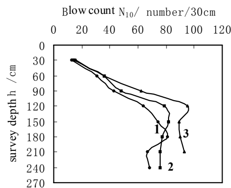
Fig.11 Relation between N_{10} and h of light dynamic petrenating
