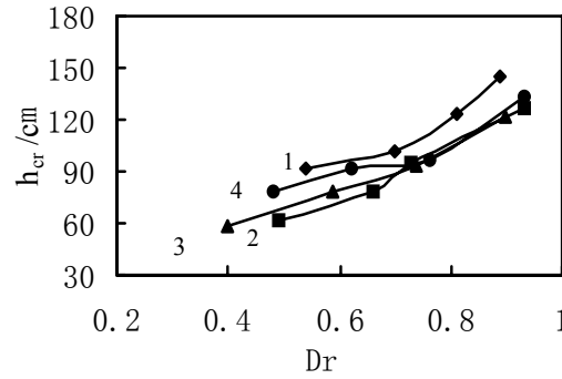
Fig.8 Calculation relation between h_{cr} and D_r
