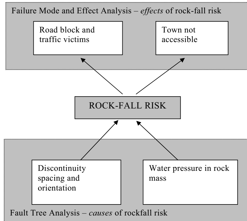
Fig.2 Combined cause and effect analysis of rock-fall risk (van Staveren, 2006)
