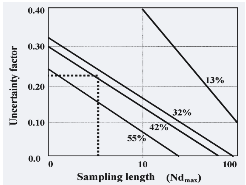
Fig. 15 Uncertainty in estimates of volumetric block proportion as a function of the length of linear measurement, expressed as a multiple ( N ) of the length of the largest block ( d_{max} ), and the measured linear block proportion (13 to 55 %). (35). The dashed line is shows the use of the graph for an example (provided in the text) at Scott Dam, where the 150 m of drill core (sampling length) was equivalent to 5 times the size of the largest block expected in the region of the dam (30 m). Hence, Nd_{max} is 5. The measured linear block proportion was 40 %. Entering the graph at Nd_{max} of 5, and intersecting the linear volumetric proportion of 40 % (interpolating between 42 and 32 % diagonal lines), gives an uncertainty factor of 0.23 (dimensionless). The uncertainty is assuming that the linear block proportion is the same as the volumetric block proportion is estimated as 40 % \pm (0.23-40 %), or 40 % \pm 9 %, giving upper and lower bounds of 31 % and 49 %. The actual volumetric block proportion will generally lie within the range of the lower and upper bounds. It is prudent to use the lowest estimate if the volumetric block proportion will be used to estimate bimrock strength. On the other hand, if the volumetric block proportion will be used for excavation purposes, it may be appropriate to overestimate the block proportion, in which case the upper bound could be used.
