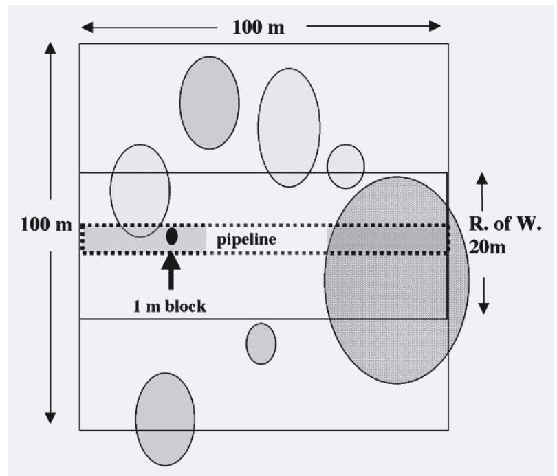
Fig. 5 Sketch showing various scales of interest for an area where a 20 m wide road and 2 m wide, 2 m deep pipeline trench will be excavated in a melange birmrock.
