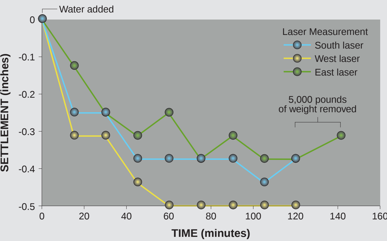
Exhibit 9 Hydroconsolidation test results Agua Caliente Cultural Museum
