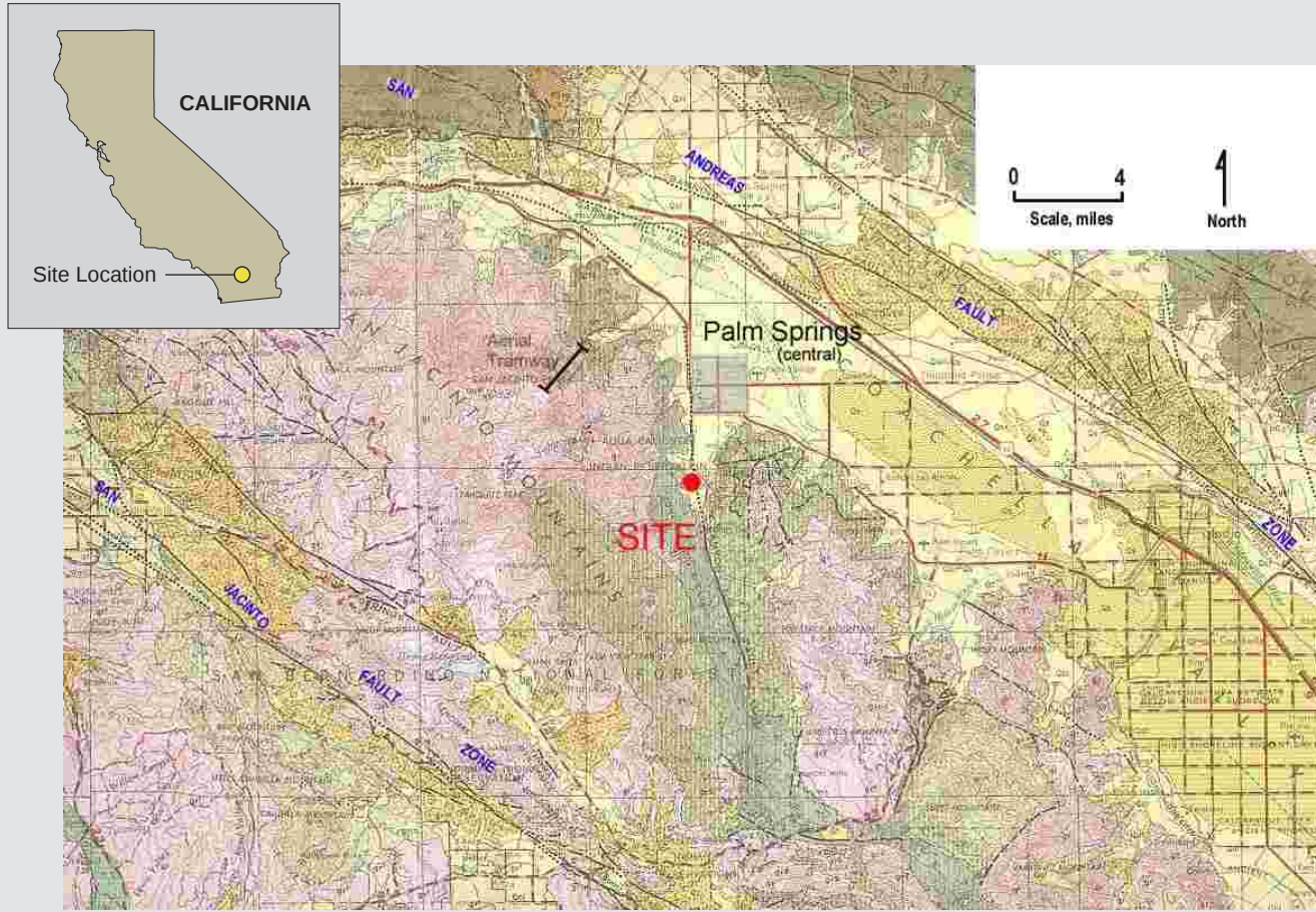
Exhibit 2 Regional geology and site location map
