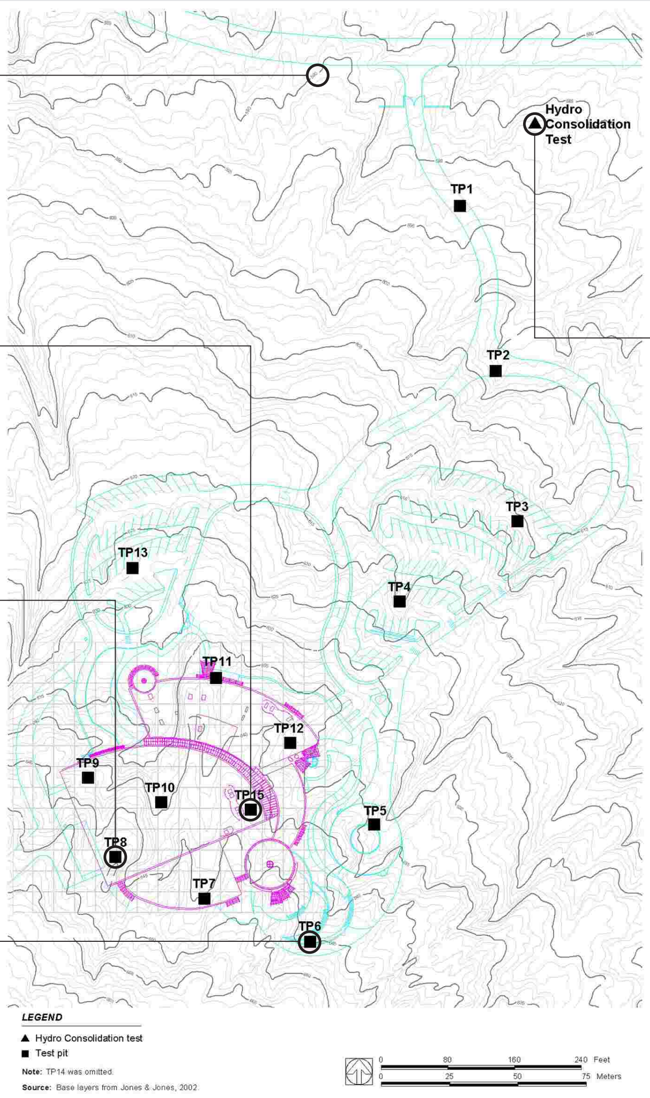
Exhibit 8 Site index map
