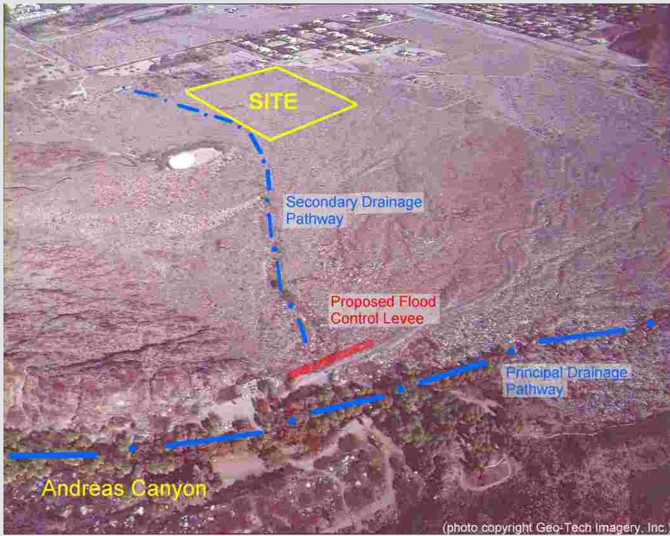
Exhibit 6 Oblique aerial photo of Andreas Canyon fan showing surface drainage features
