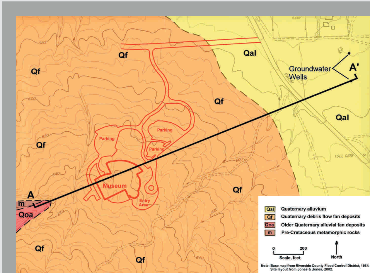
Exhibit 3 (top) Site geologic map
