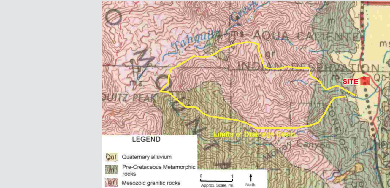
Exhibit 5 Geologic map of the Andreas Canyon drainage basin
